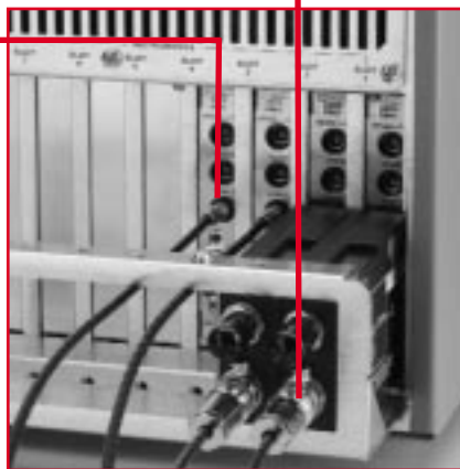
4200-SCS Rear Panel Connections
